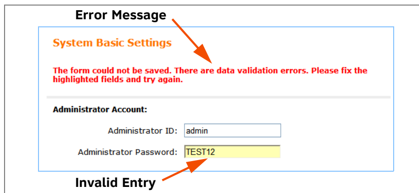
Figure 16. WebUI Error Indication
