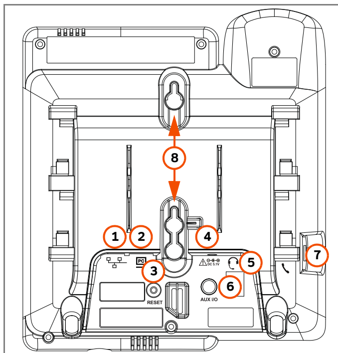
Figure 9. Deskset Connections (SB35025 Model Shown)
